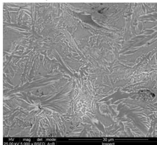
Fig 10. Microstructura zonei topit (5000x).
